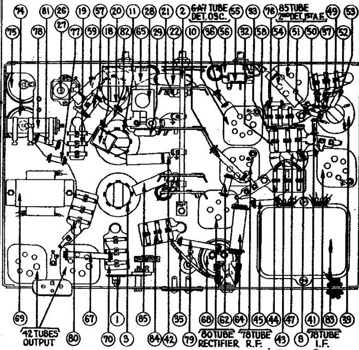
Fig. 3. Bottom View of Chassis
