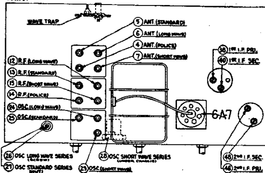
Fig. 2. Locations of Compensating Condensers
