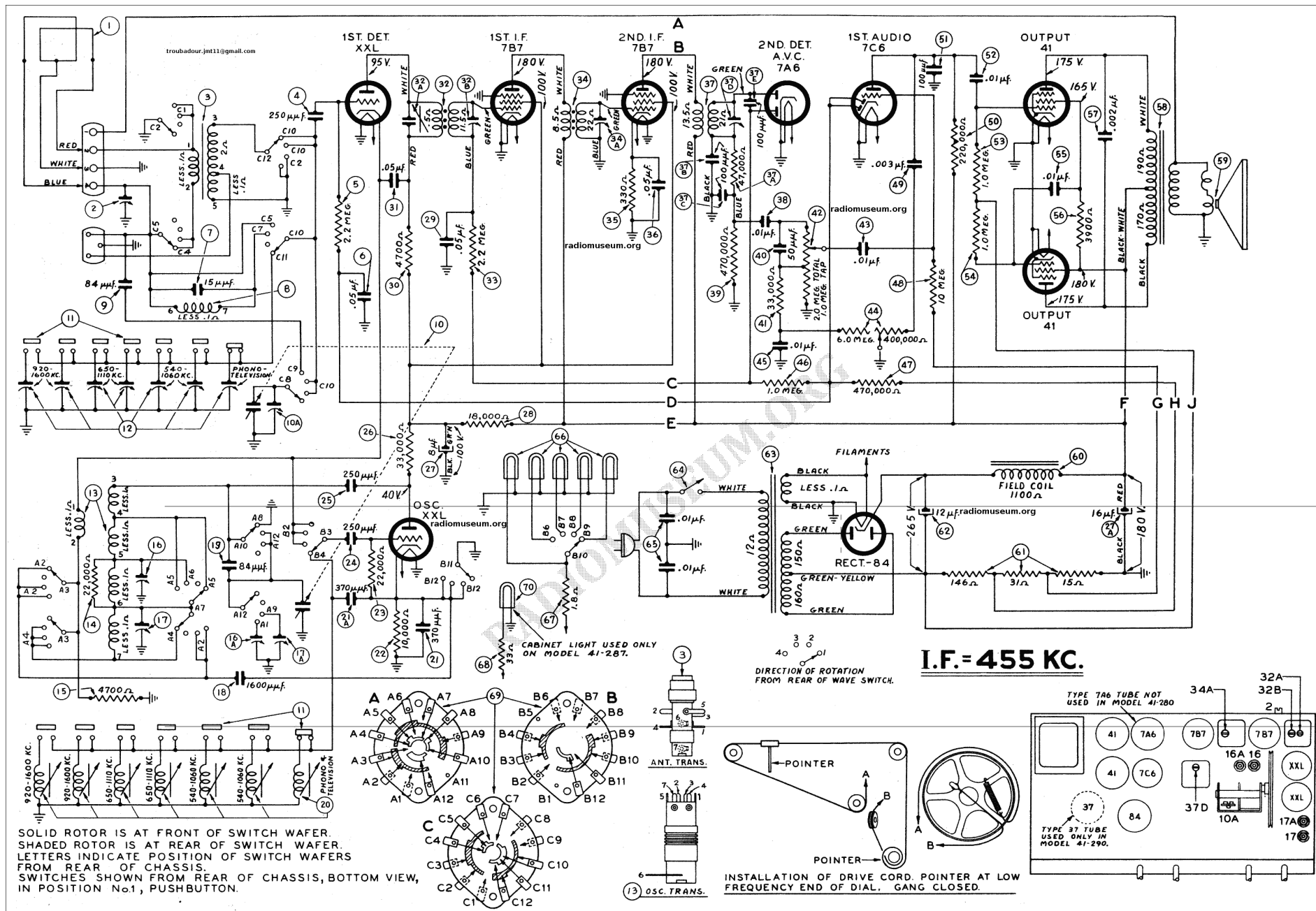
SCHEMATIC DIAGRAM — MODELS 41-280, 41-285, 41-287, 41-290
