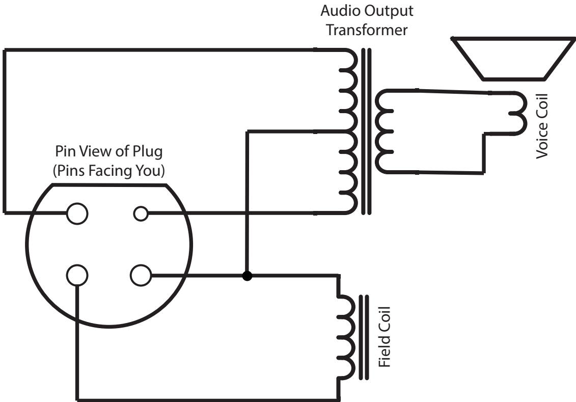
Philco 90 Early - Speaker Assembly (Push-Pull 45 Output Tubes)
